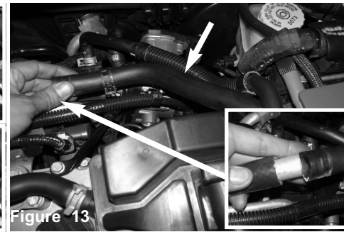
Figure 13 Reposition the crankcase line under the additional ventilation line. With provided 5/8" aluminum coupler, connect the 15mm hose provided to the original crank case line and secure.
