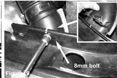
Figure 9 Loosen the bolt holding in the snorkel scoop on the radiator support. Now pull back the snorkel scoop from the radiator support.
