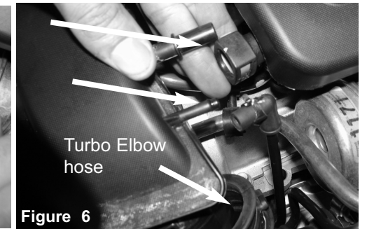
Figure 6 Disconnect the vacuum lines from the stock intake tube. Now lift up and pull the stock intake tube out of the stock turbo elbow hose. Leave the hose on turbo.
