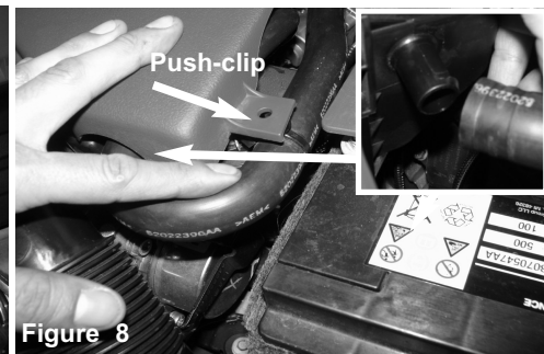
Figure 8 Now push the clip holding in the crank-case line away from the air-box/engine cover. Pull back the crank-case line from the air box.
