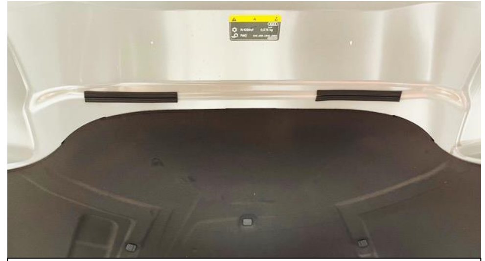
39. Take the 2 rubber strips provided and stick them to the underside of the hood as shown. These protect the carbon from contact with the hood. The should sit on the curved surface of the hood.
